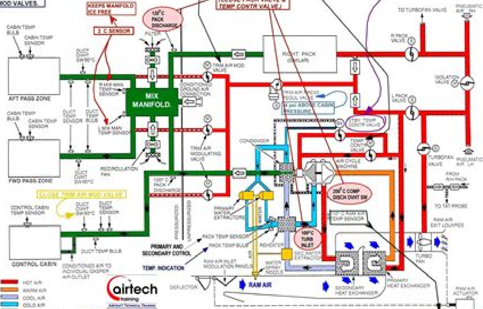
Figure 26 Air Conditioning System Schematic
