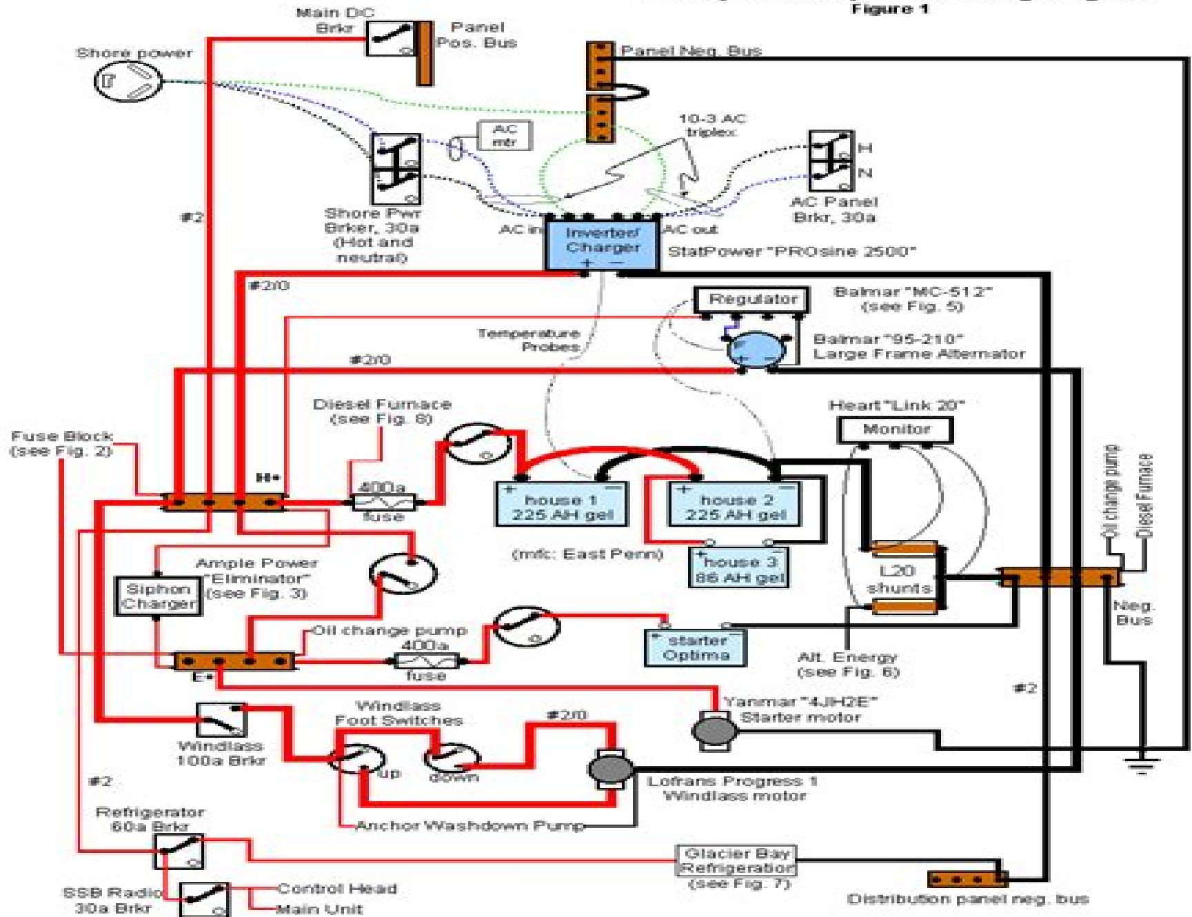
Primary Power Systems Wiring Diagram
