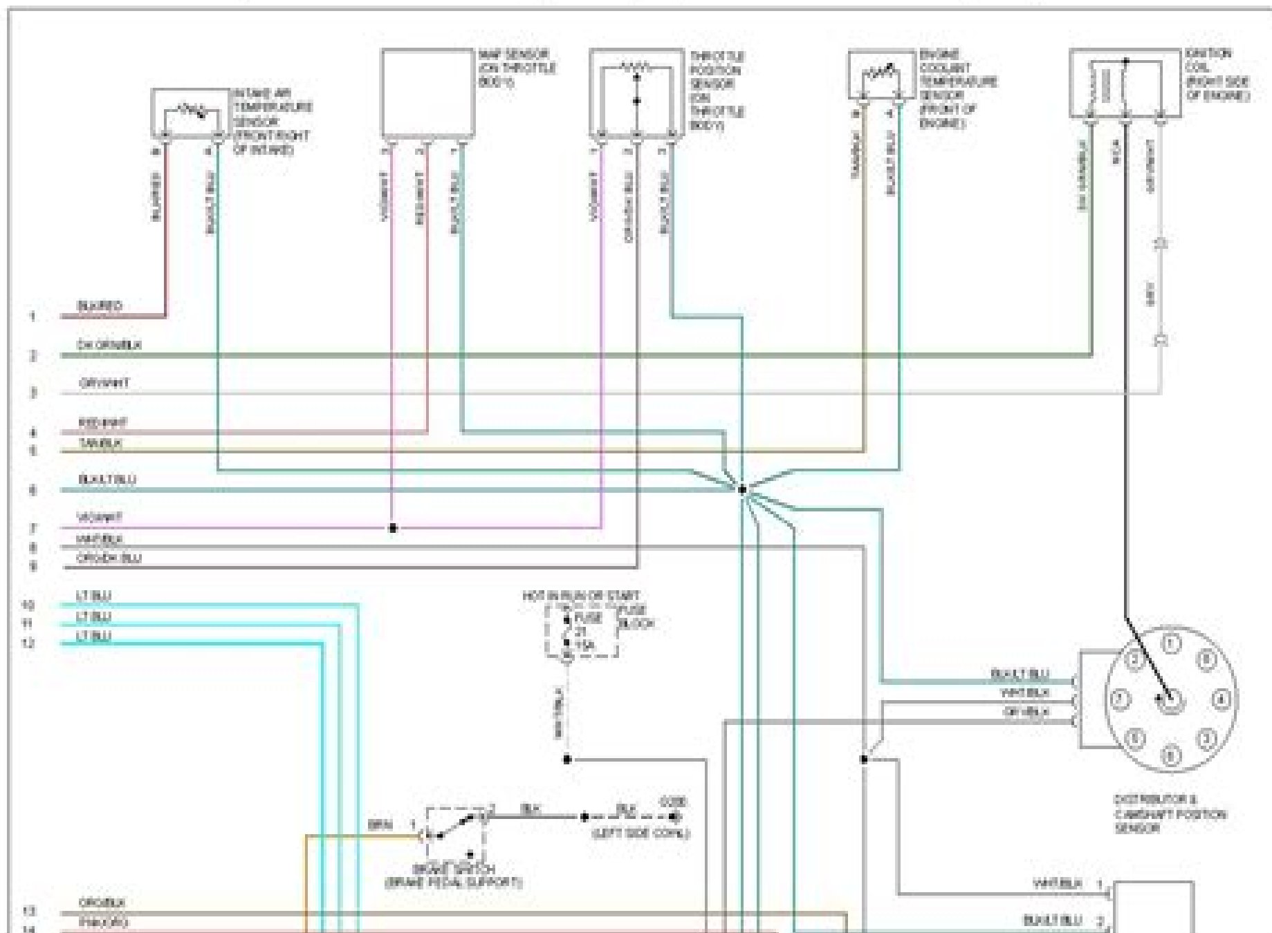
1994 Jeep Grand Cherokee Laredo-Fig. 9: 5.2L, Engine Performance Circuits (2 of 2)
