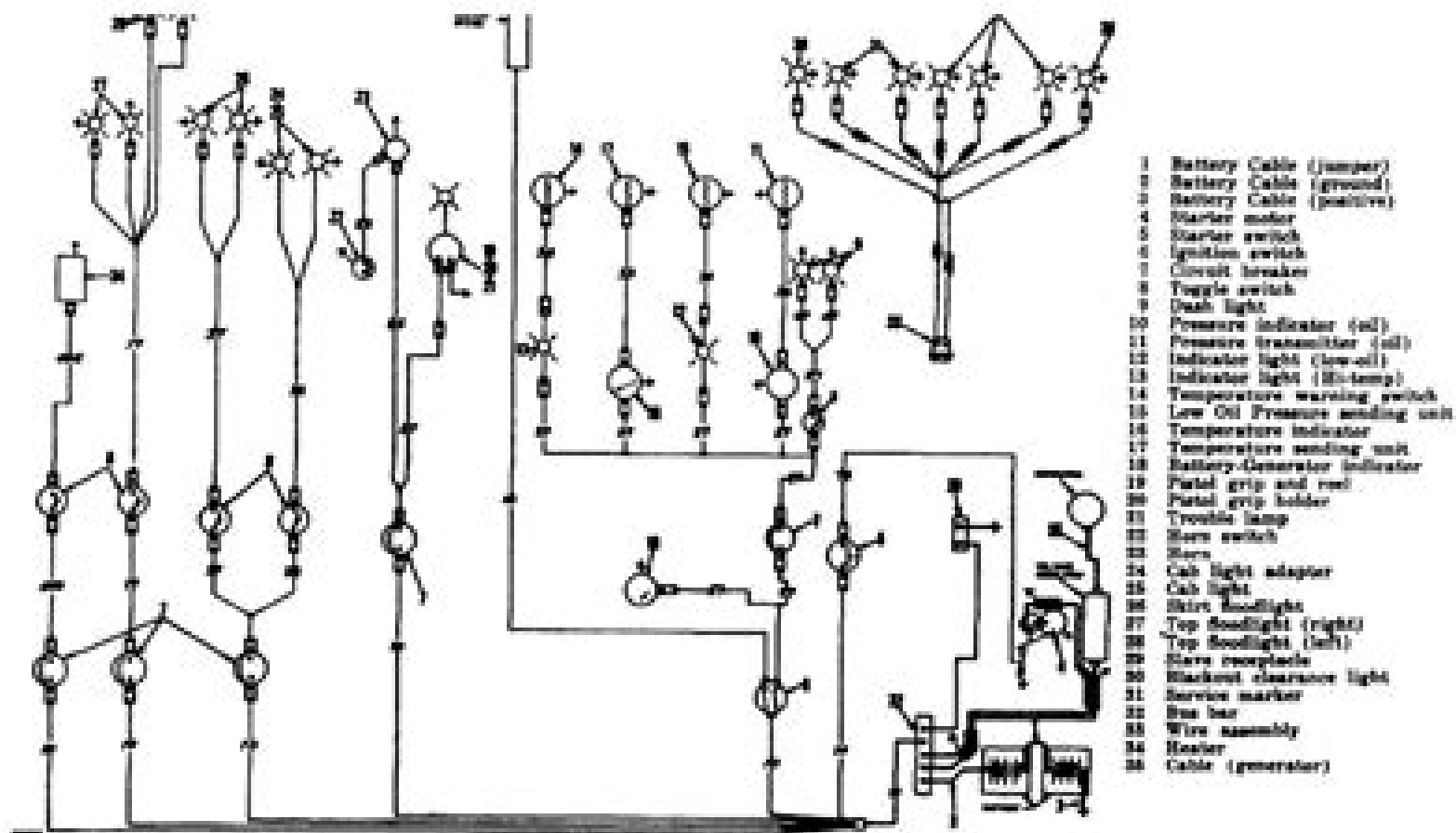
B - Crane Wiring Diagram.
