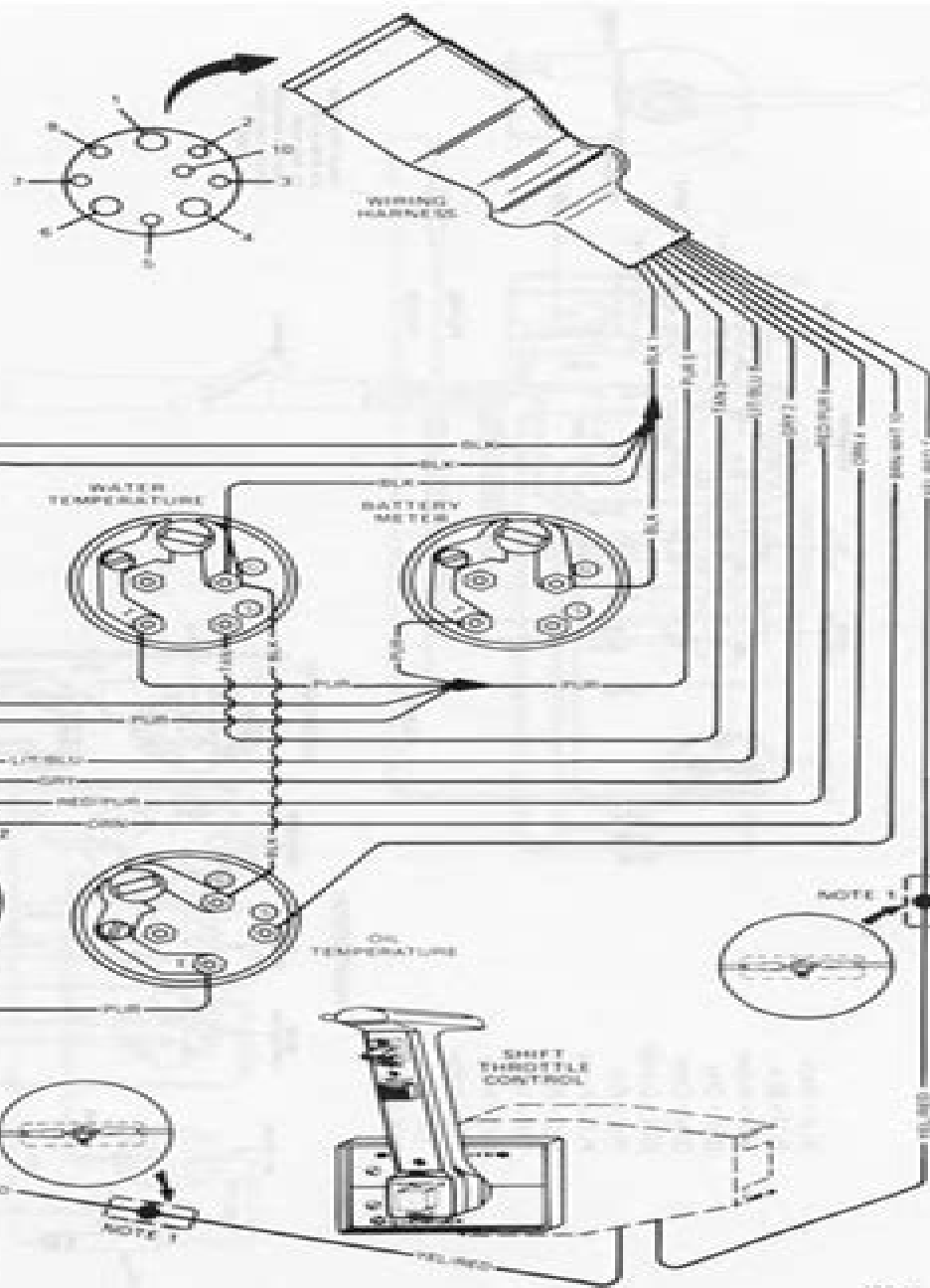
Quicksilver Engine Instrumentation
