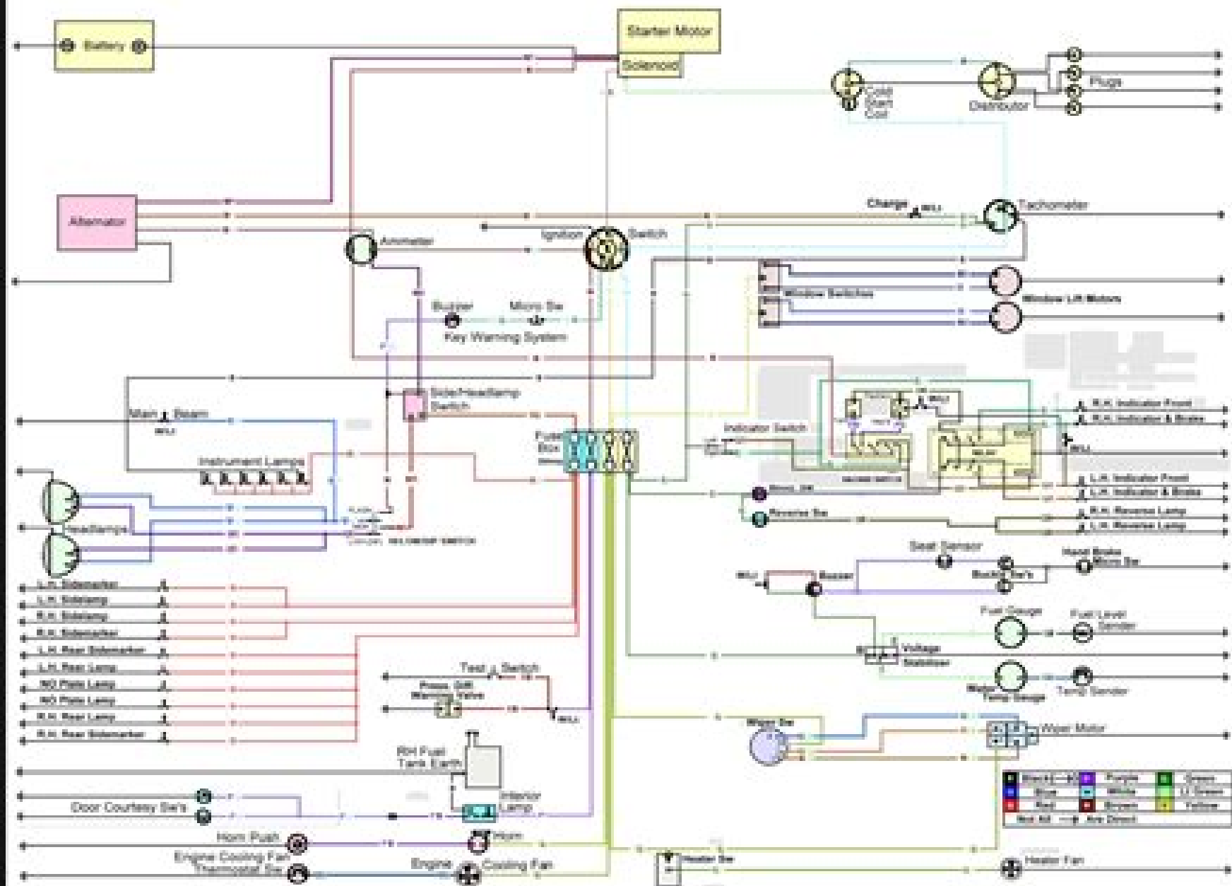
Europa Twin-Cam Wiring Diagram (Federal)
