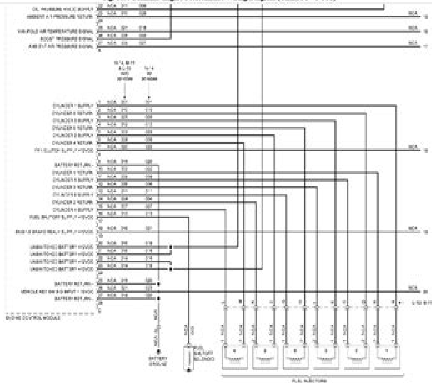
Fig. 139: Cummins Engine Performance Wiring Diagram (CELECT - 1 OF 3)
