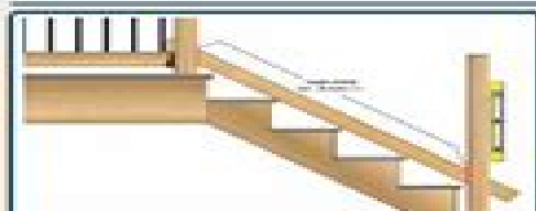
STEP #1 - Lay bottom rail alongside posts and mark for angle. If posts are plumb top rail should be the same length and angle. Cut top and bottom stair rails at proper angle.
