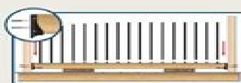
STEP #5 - Install two (2) #8 x 2" screws (per connector) through railing connector into rail ends. Rest bottom rail on two (2) temporary spacer blocks the required height between deck and bottom of bottom rail. Center railing connectors on post and install four (4) #8 x 2" screws (per connector) through railing connector into posts. Apply a small amount of silicone caulk to diameter of baluster where it meets baluster connector or insertion hole to insure a tight, movement free installation. Install balusters on bottom rail.
