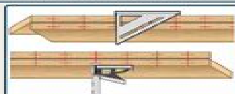
STEP #2 - Lay top and bottom rails beside each other with the top rail turned upside down. Position rails as shown. Find the center of rails and mark lightly. Measure out 5-1/2" from both sides of center line and mark lightly. End spacing will vary. Set a combination square for center (example: 1-1/2" = 3/4") and mark lightly. Where lines intersect will be center of screw/insertion hole.
