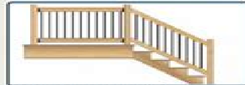
STEP #8 - Install stair rail assembly.
