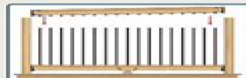
STEP #6 - Start Top Rail at an angle and insert connectors into balusters or balusters into insertion holes in top rail. Make sure balusters are fully connected. Install four (4) #8 x 2" screws (per connector) through railing connector into posts.
