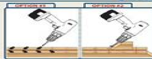
STEP #6 - There are two options for installing balusters. Option #1 - Connector Method: Insert screw through connector and install where lines intersect (nail hole is now vertically and tilt screw to proper angle. Top and bottom baluster connectors will be facing opposite directions. Do not over-tighten. Option #2 - Insert Method: Drill a 3/4" hole, 3/8" deep in top and bottom rails where lines intersect using a nail cut-off as a guide block for rail angle.
