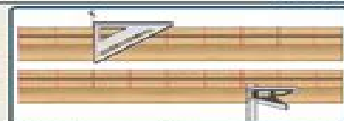
STEP #3 - Lay top and bottom rails beside each other and flush ends. Find the center of rails and mark lightly. Measure out 4-1/2" from both sides of center line and mark lightly. End spacing will vary. Set a combination square for center (example: 1-1/2" = 3/4") and mark lightly. Where lines intersect will be the center of baluster.
