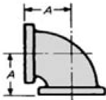
90 deg. Elbow
