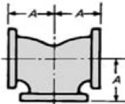
Double-Branch Elbow
