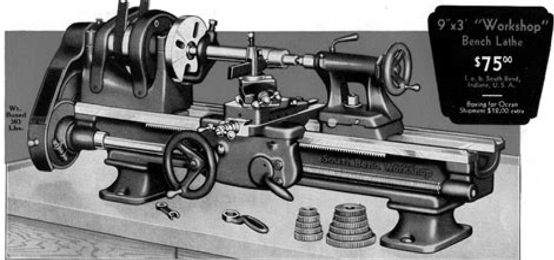
Fig. 1. 9" x 3' No. 5-YB, "Workshop" Bench Lathe Complete as Shown with Regular Lathe Equipment.....$75.00
