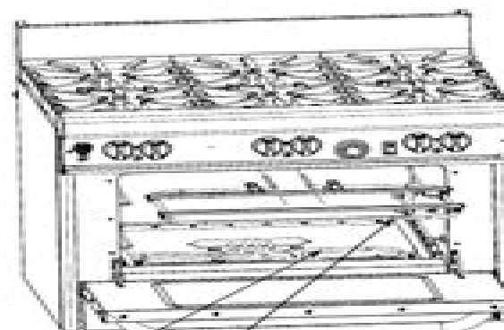
Top Element (Standard Oven) 208V P/N 1191621 240V P/N 1191622 480V P/N 1191625
