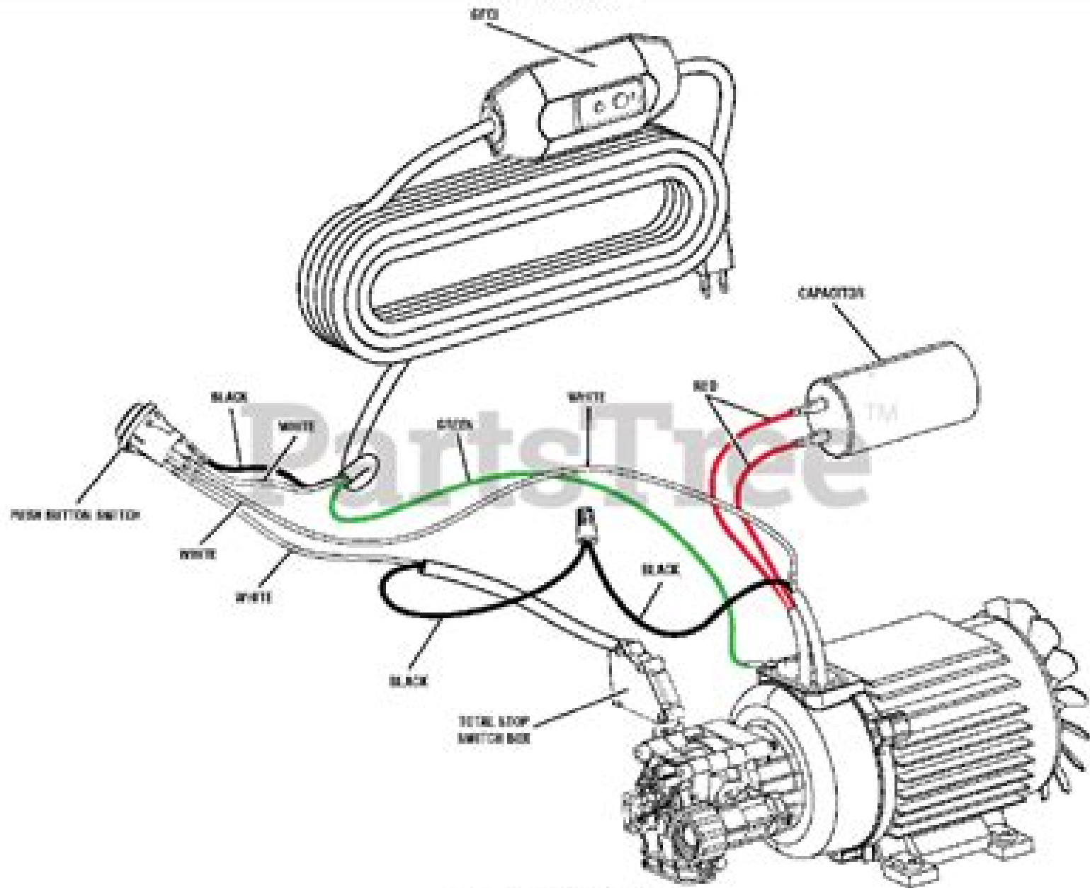
WIRING DIAGRAM
