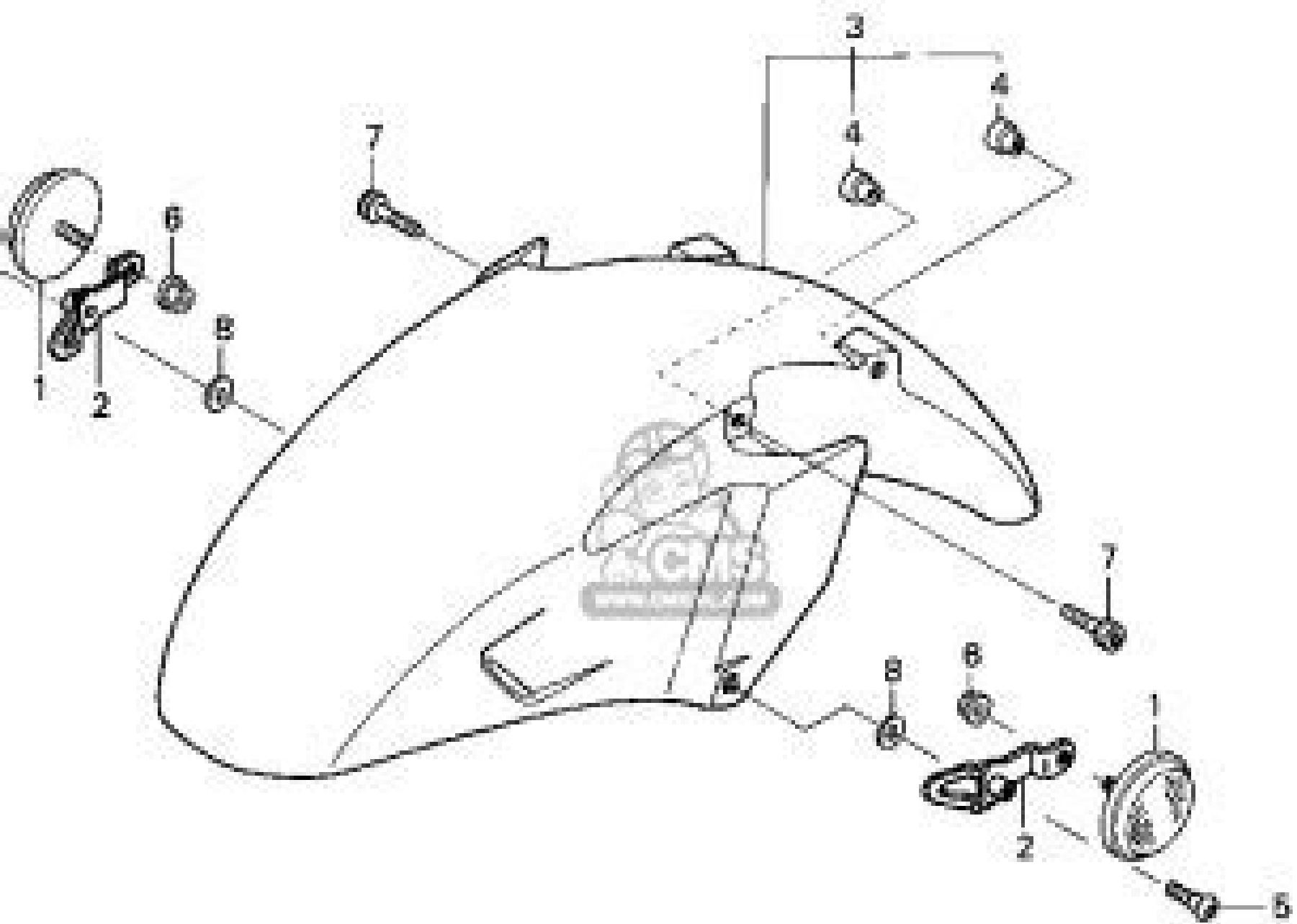
FRONT FENDER
