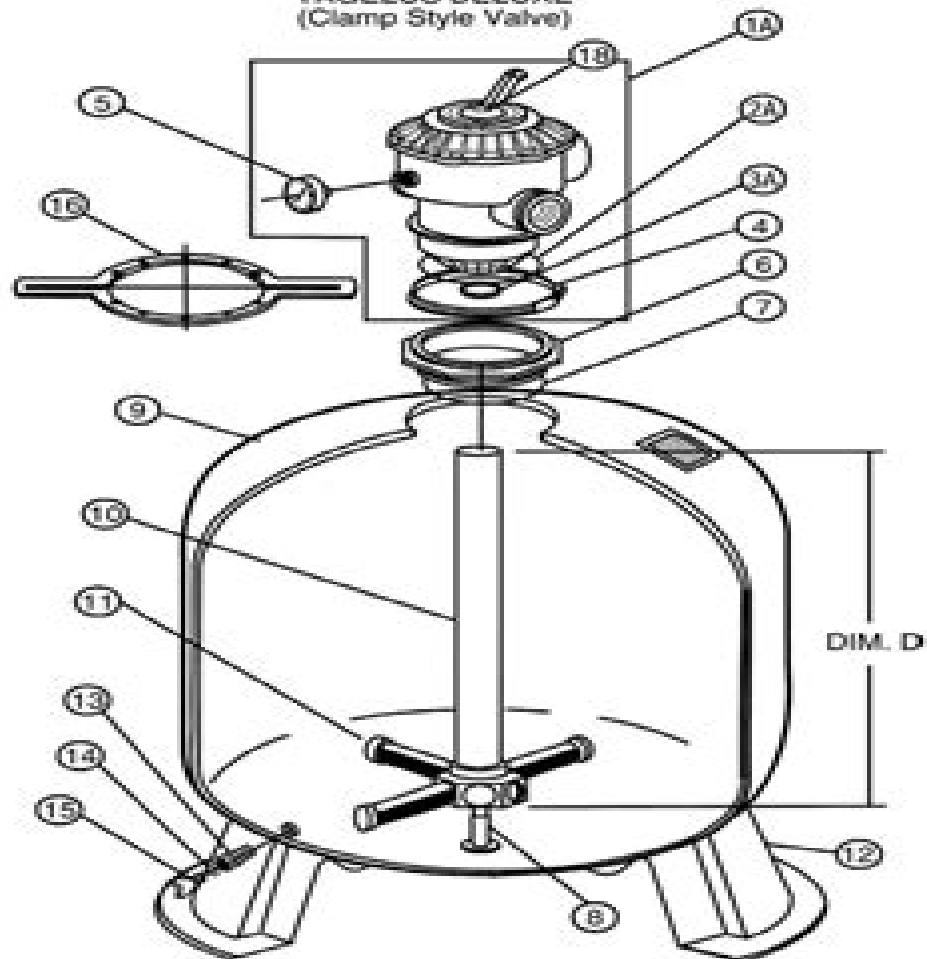
TAGELUS DELUXE (Clamp Style Valve)
