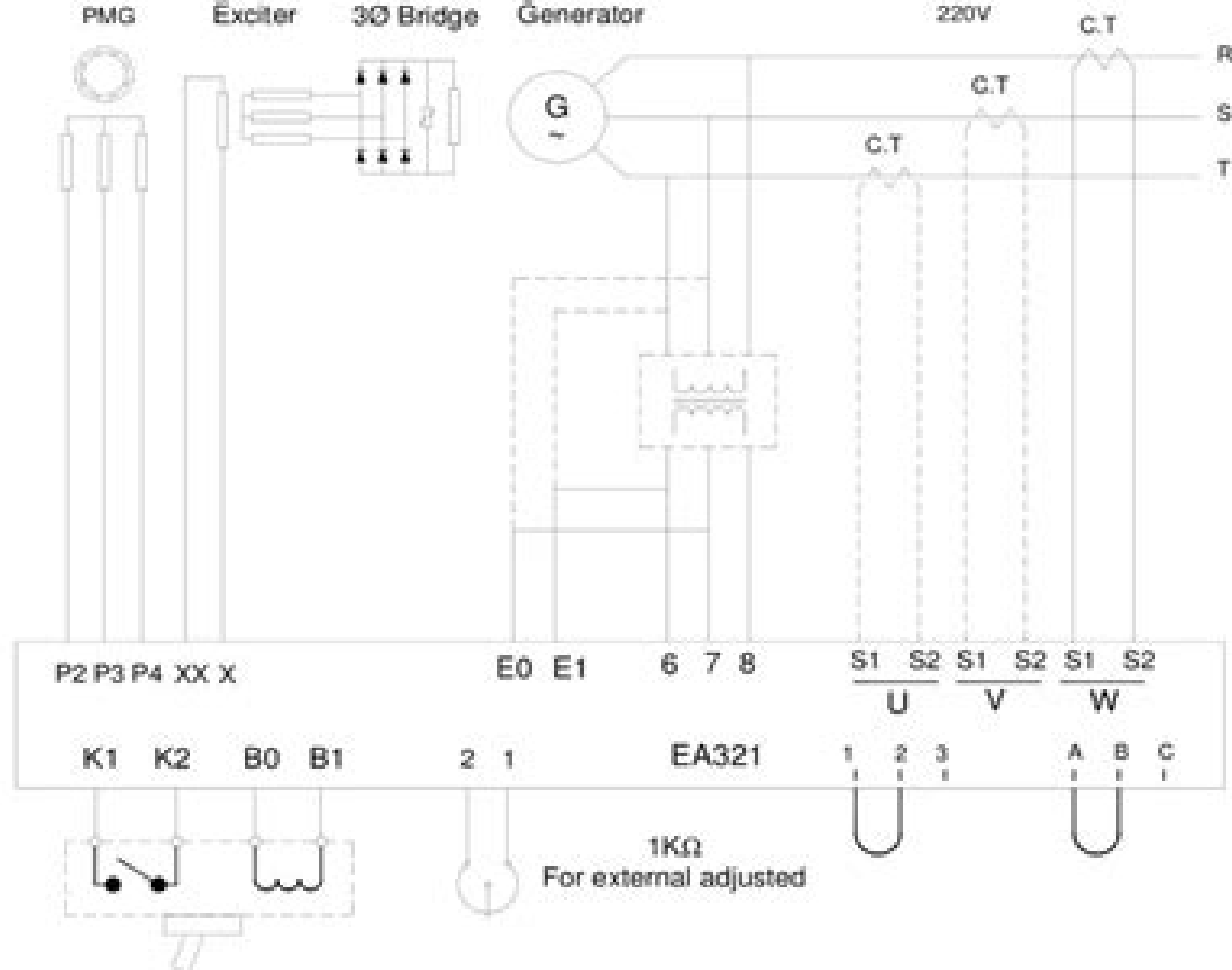
Figure 3 Wiring Drawing
