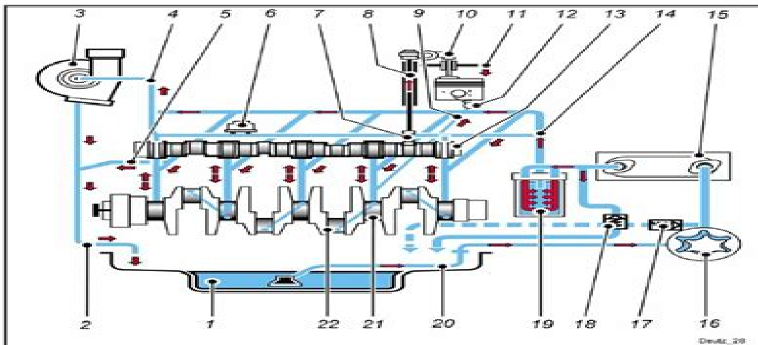
Fig. 1 Lubrication oil circuit
