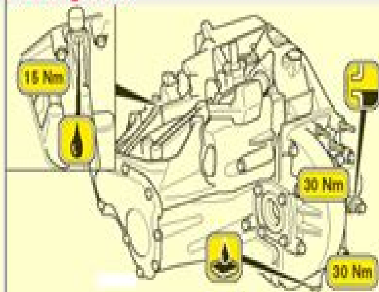
Manual gearbox
