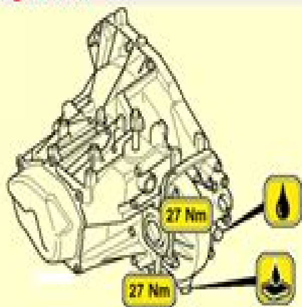
Manual gearbox
