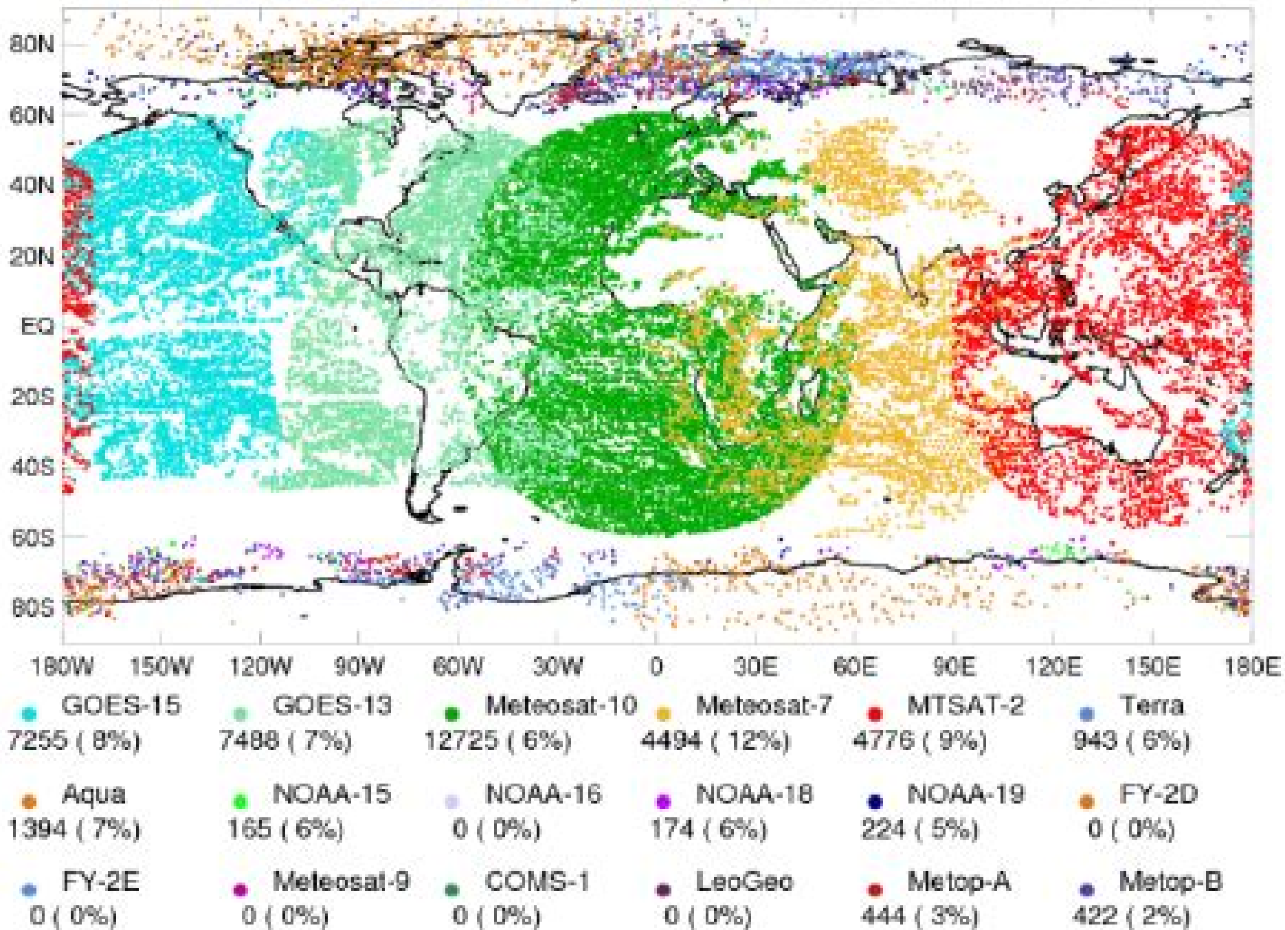
Location of used AMVs, all levels, 12z 02 November 2014
