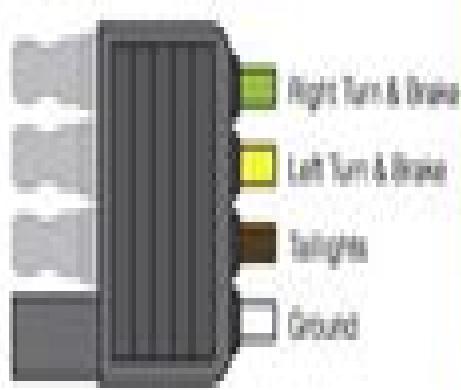
4 Wire Flat
