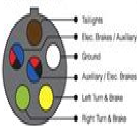
6 Pole Round
