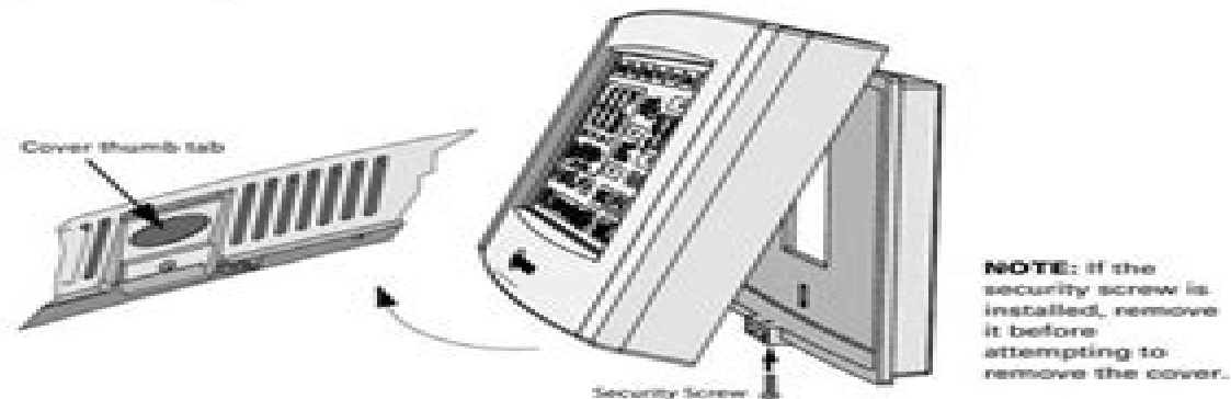
Figure 1. Security screw removal and cover release
