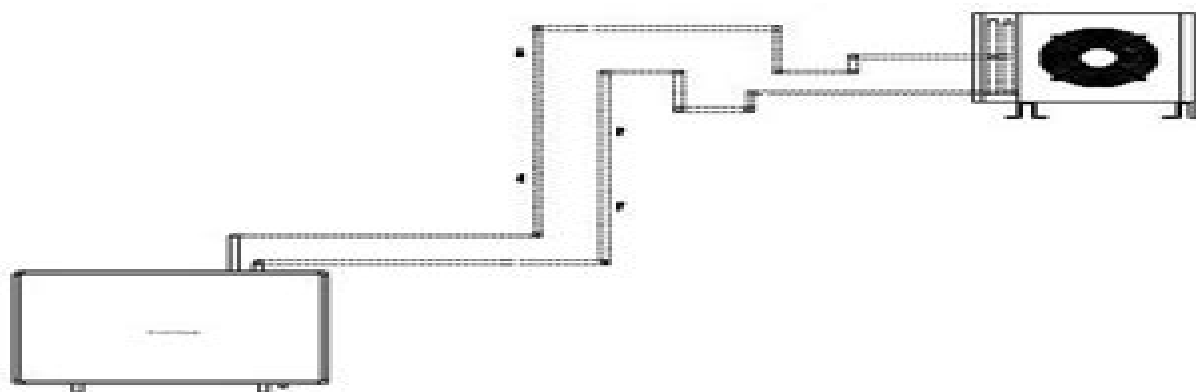
Dehumidifier lower than condenser
