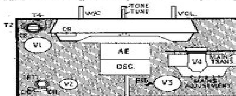
Layout diagram of the MP chassis (condensate on right) identifying components. Condensers are in outline and resistors in solid black to aid reference.
