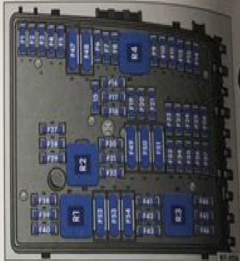
Fig. 51 Fuses in the engine compartment fuse box for the Golf GTI
