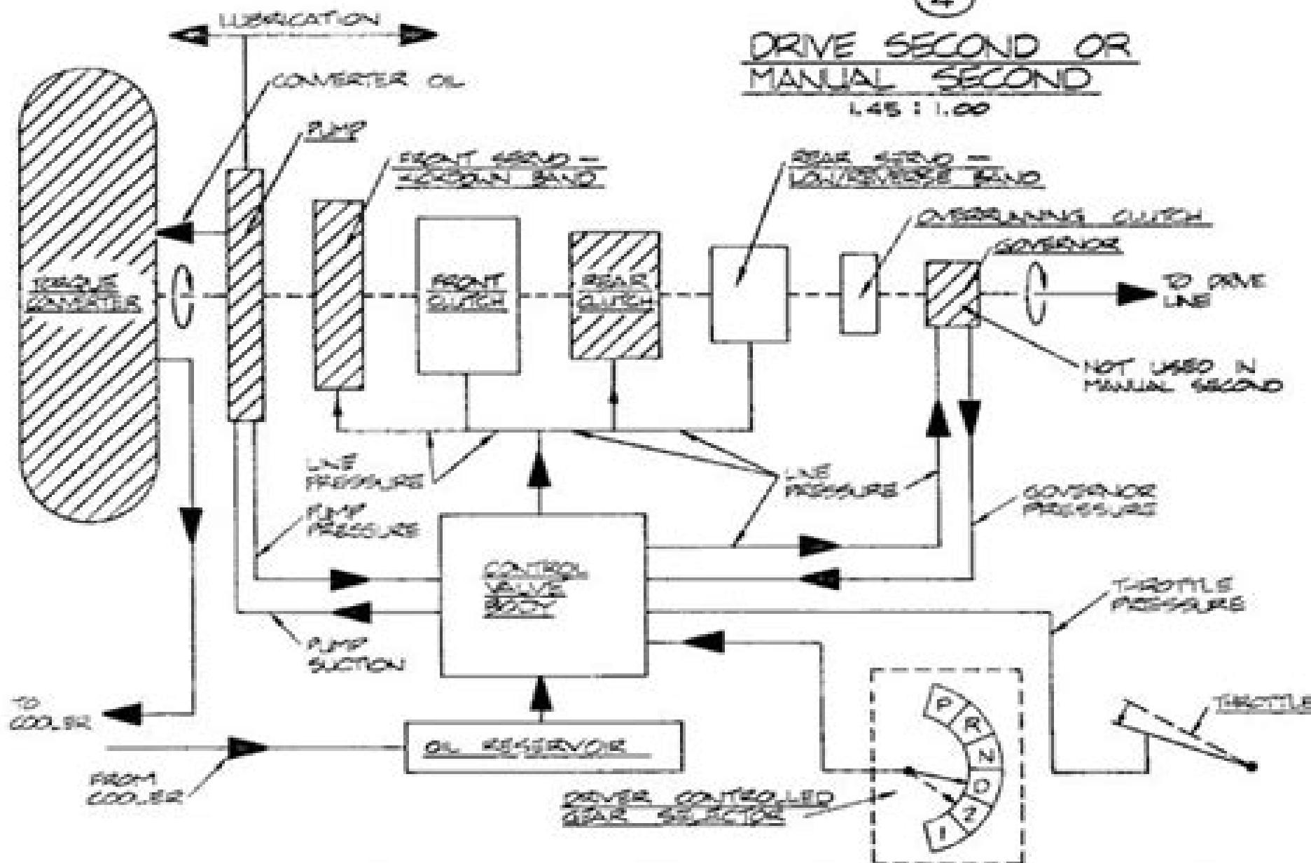
TORQUEFLITE TRANSMISSION BLOCK DIAGRAM
