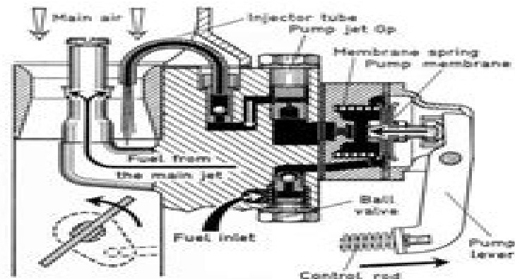
Fig. 29 Mechanically operated accelerator pump
