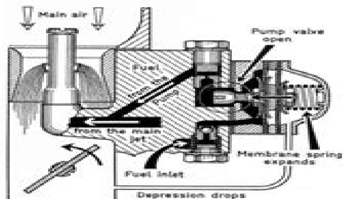
Fig. 30 Depression-operated accelerator pump
