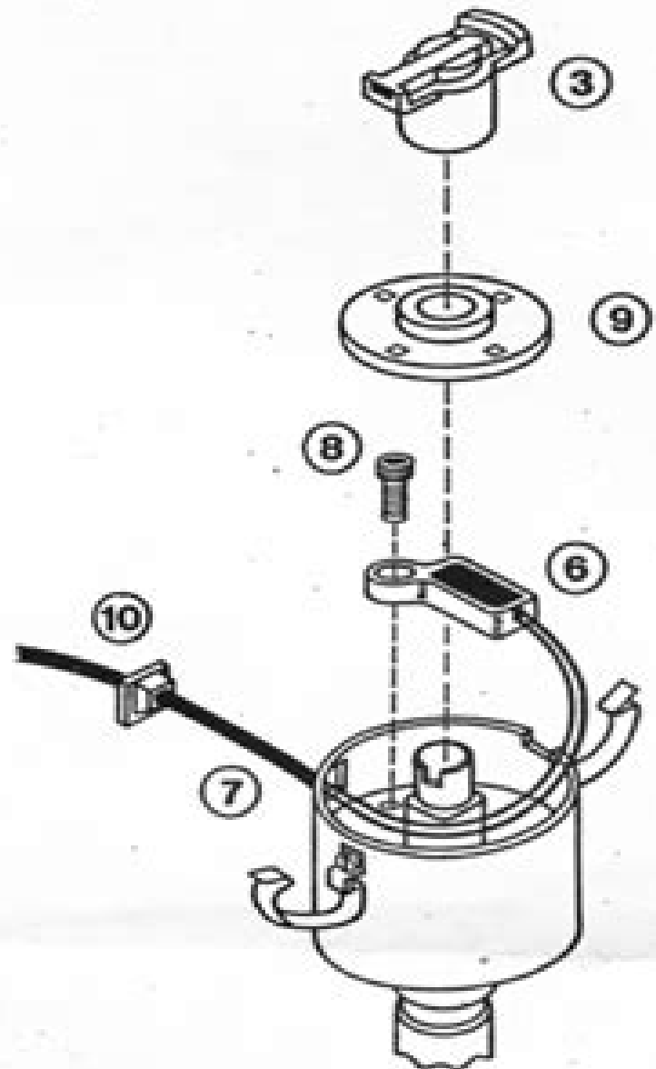
COMPU-FIRE INSTALLATION FIGURE 2
