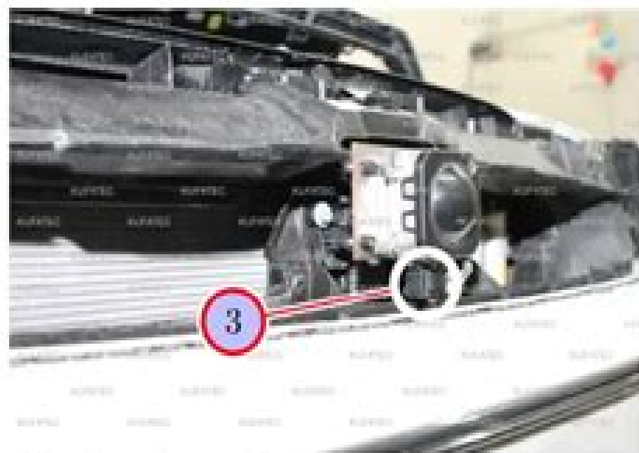
Figure 2: Removing front grille / replace radar sensor
