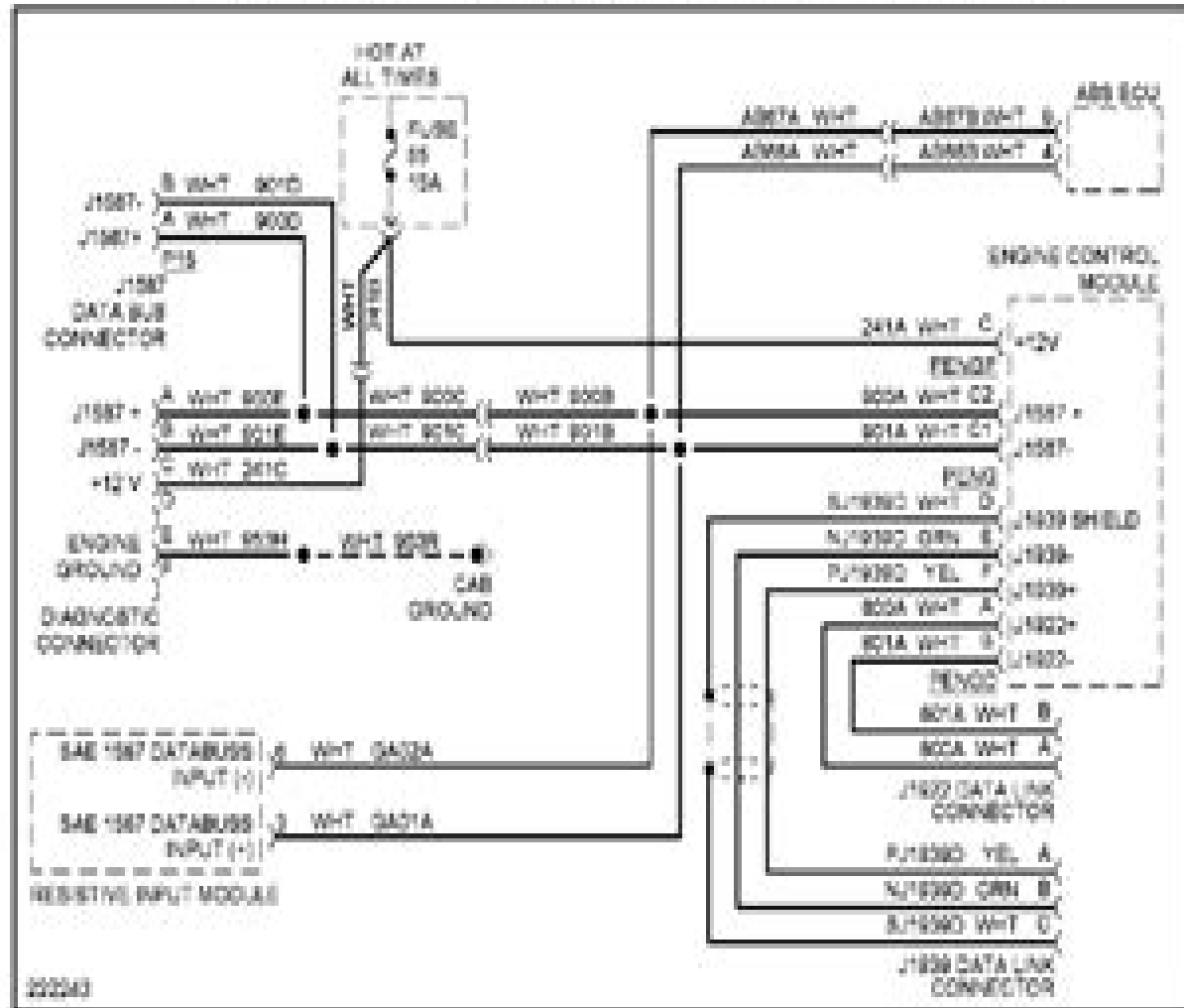
Fig. 126: Computer Data Lines Circuit, DDEC III Series 60 W/BOM Serial Number 3463
