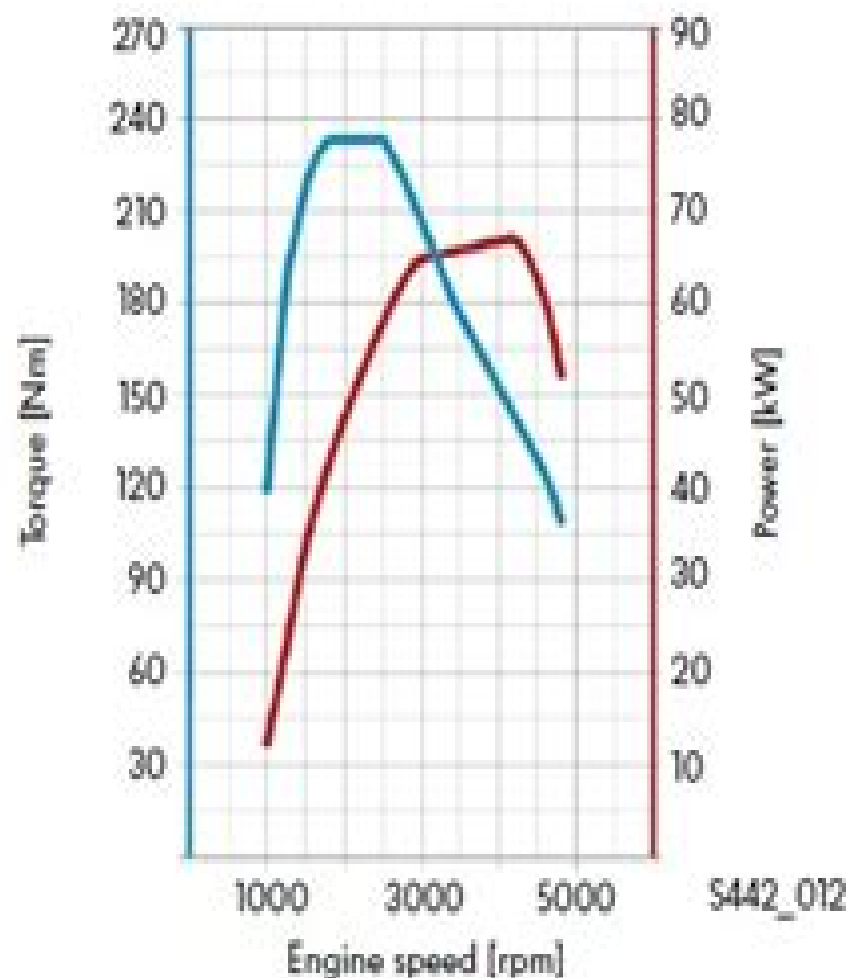
Torque and output diagram
