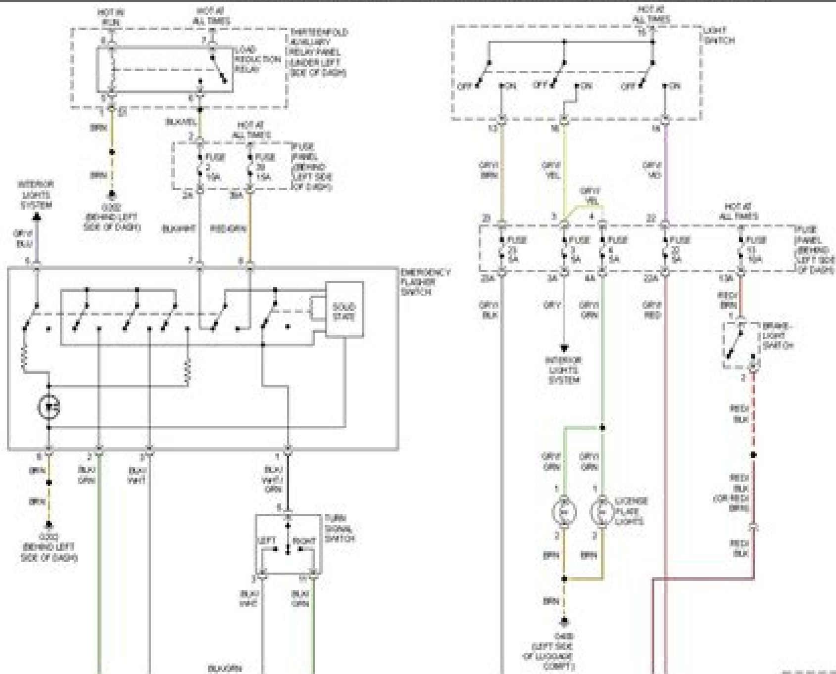
2001 Volkswagen Jetta GLS-Fig. 42: Exterior Lamps Circuit
