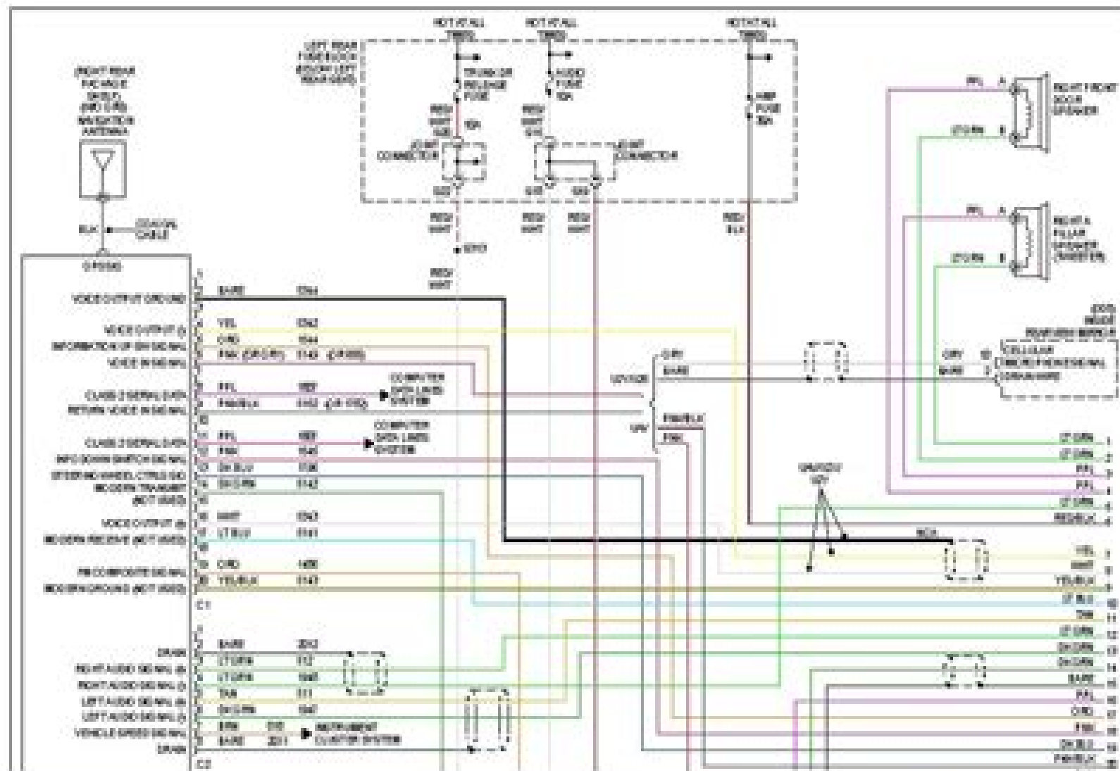
2004 Cadillac CTS-Fig. 70: Radio Circuit, Luxury (1 of 2)
