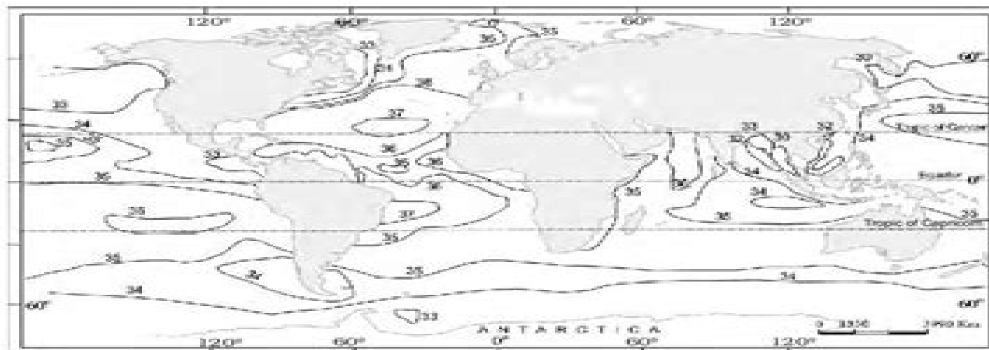
Figure 13.5 : Surface salinity of the World's Oceans
