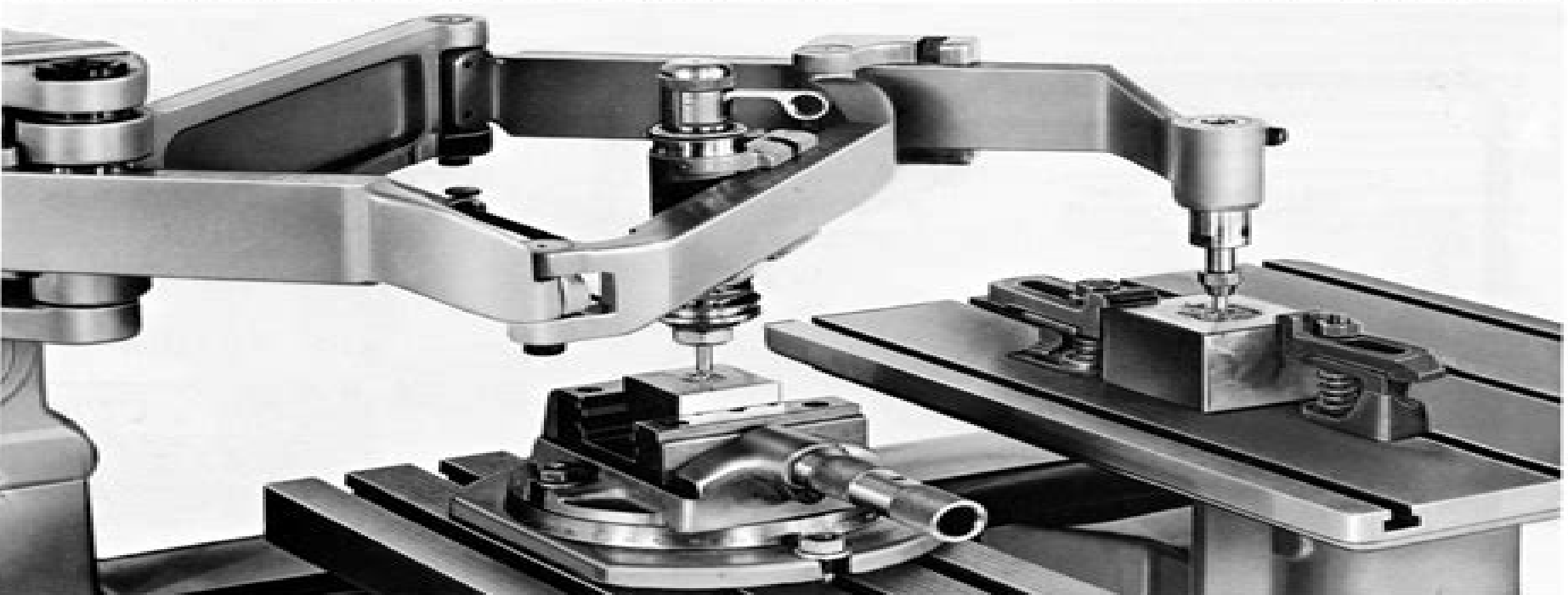
Fig 6 Reducing an escutcheon die from a steel master (GK 12)
