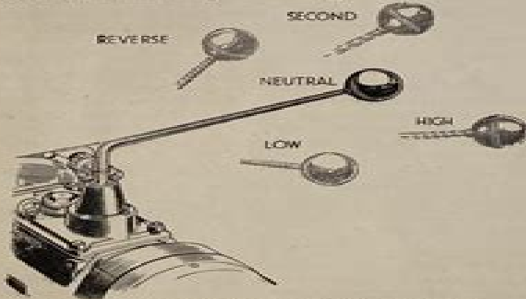
The gear positions of the 3-speed synchromesh gearbox.
