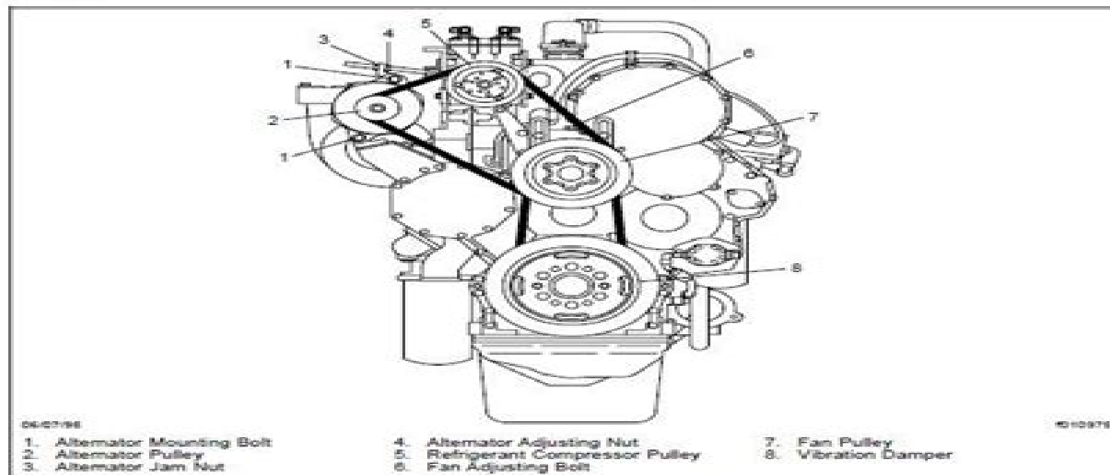
Fig. 1. Drive Belts, Caterpillar 3406
