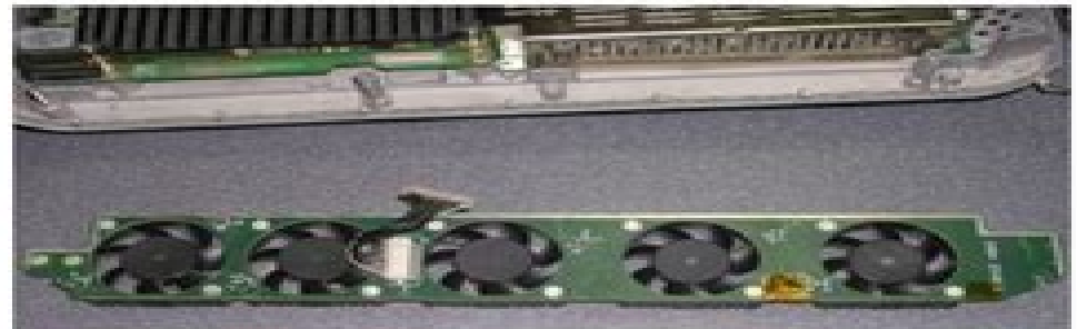
Figure 8-68 Disconnecting the Fan Cable from the BEP
