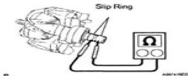
Fig. 32: Measuring Resistance Between Slip Rings
