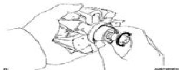
Fig. 31: Checking Bearing
