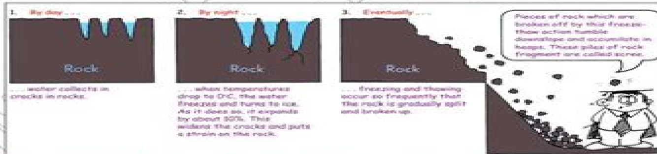
Figure 2.16 The breaking of rocks by the action of frost
