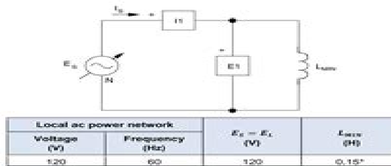
Figure 4-2. Inductive ac circuit.
