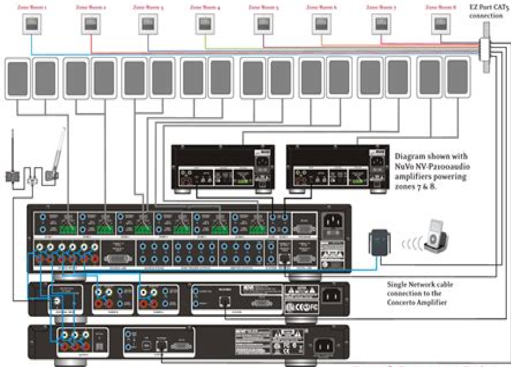
Grand Concerto Suite Wiring Diagram
