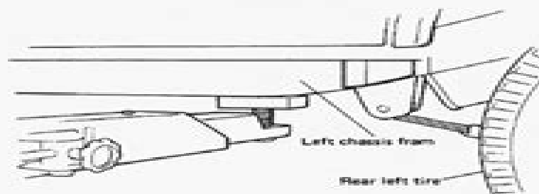
Fig. 0-8 Rear Support Location
