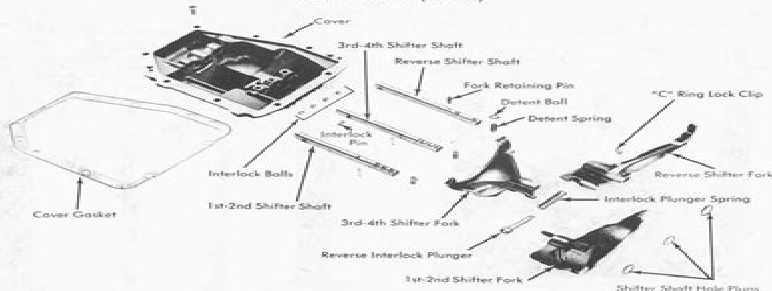
Fig. 6 Exploded View of Cover and Shift Assembly
