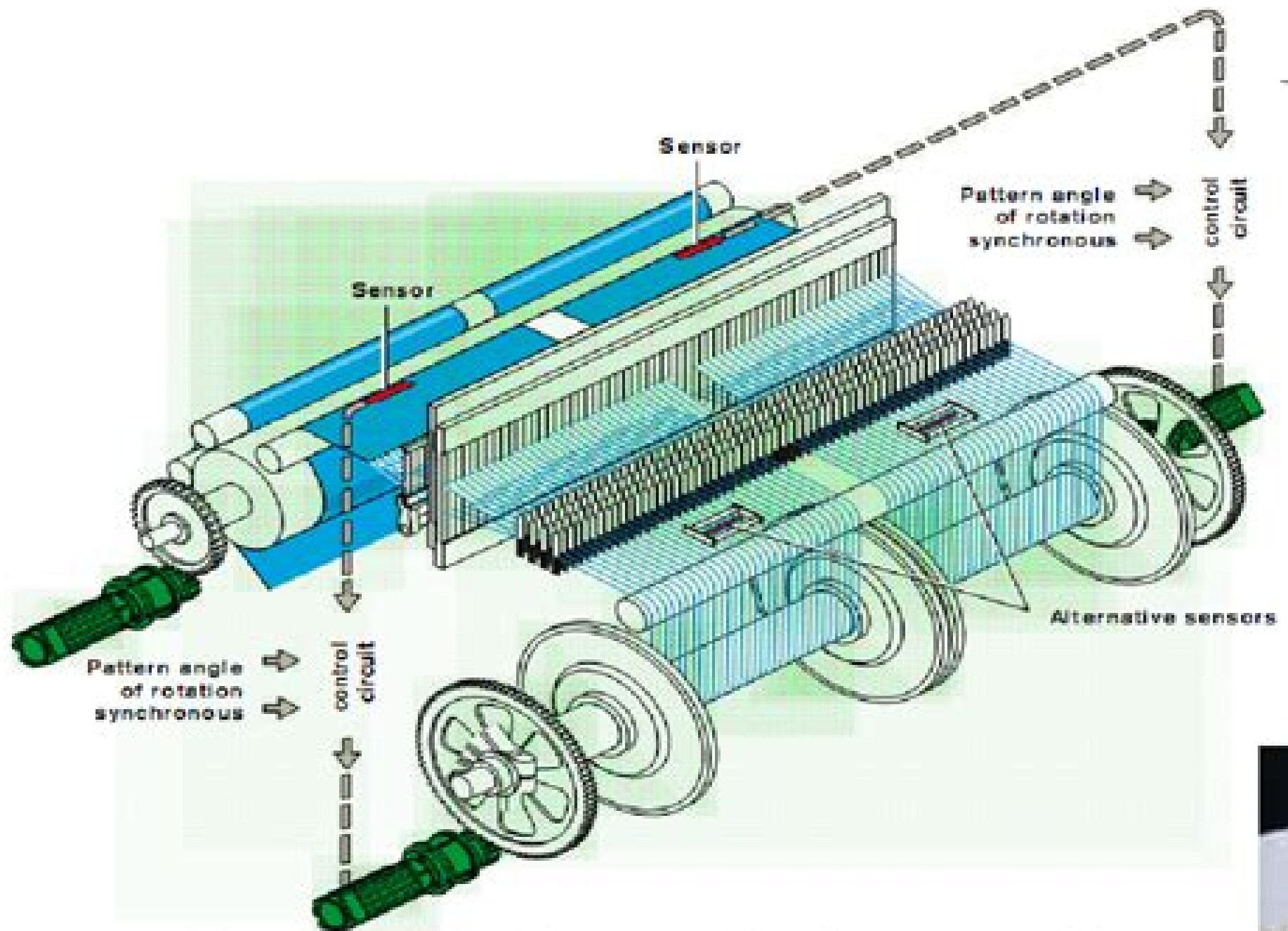
Figure 3. Synchronized Electronic Let-off and Take-up mechanism[7]
