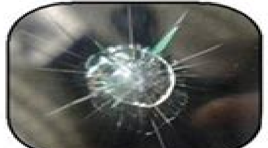
Stars
