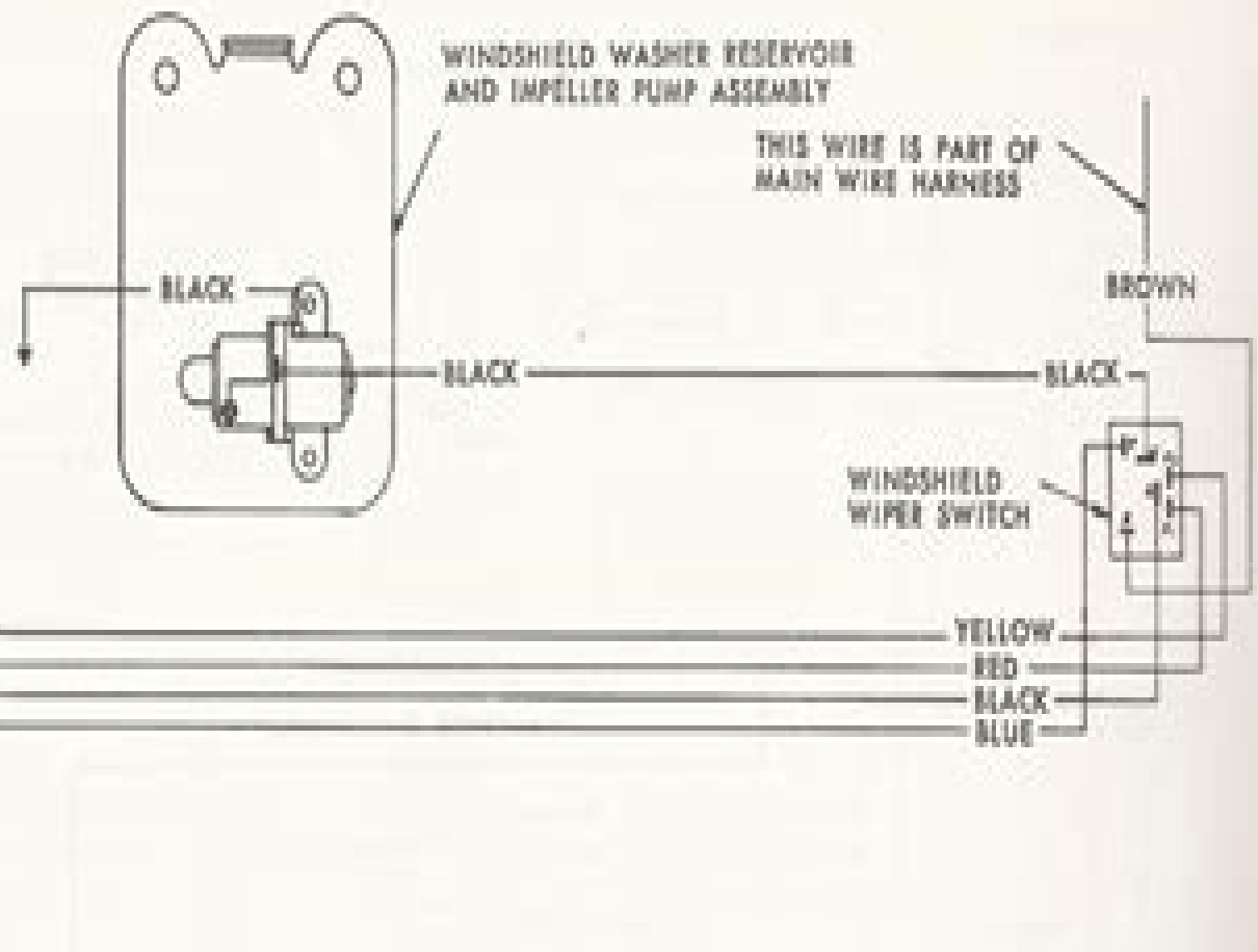
Electric Windshield Wipers and Washer Wiring
