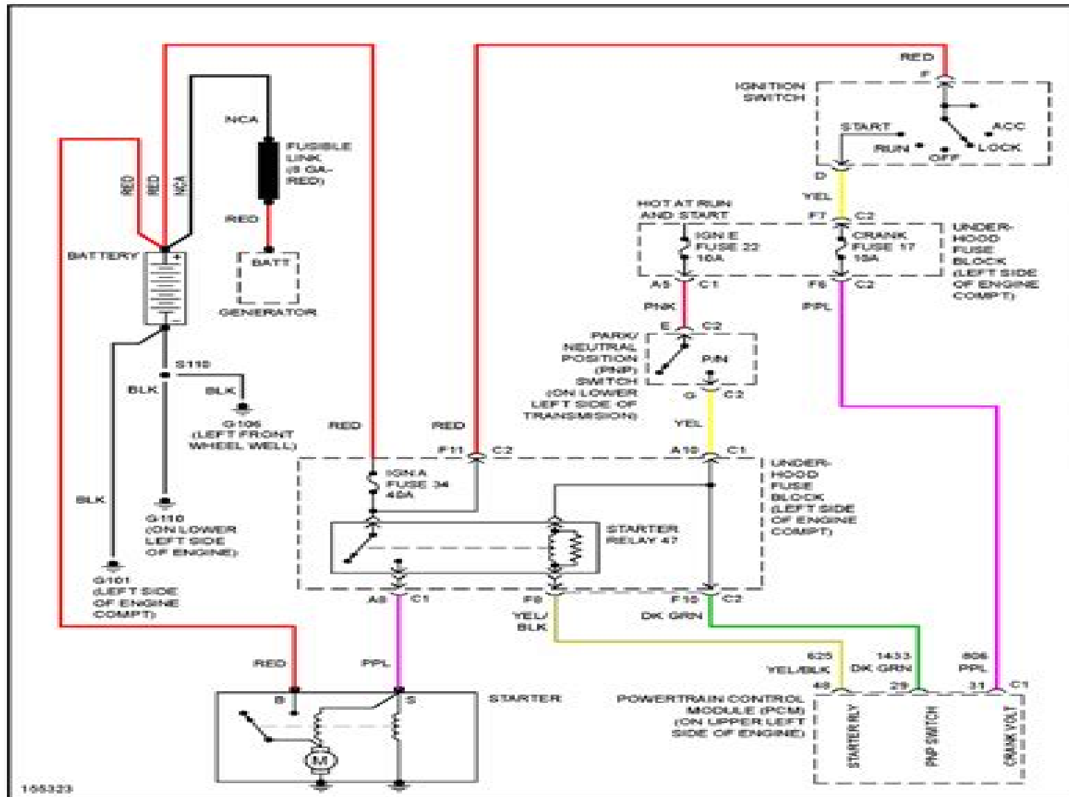
Fig. 69: Starting Circuit
