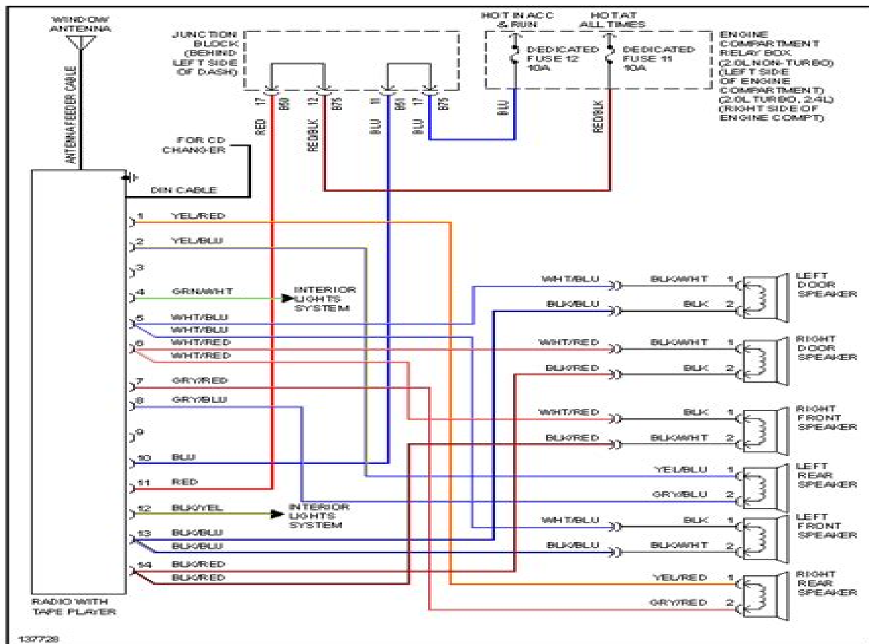
1995 Mitsubishi Eclipse GS-Fig. 49: Radio Circuits, W/O Amplifier
