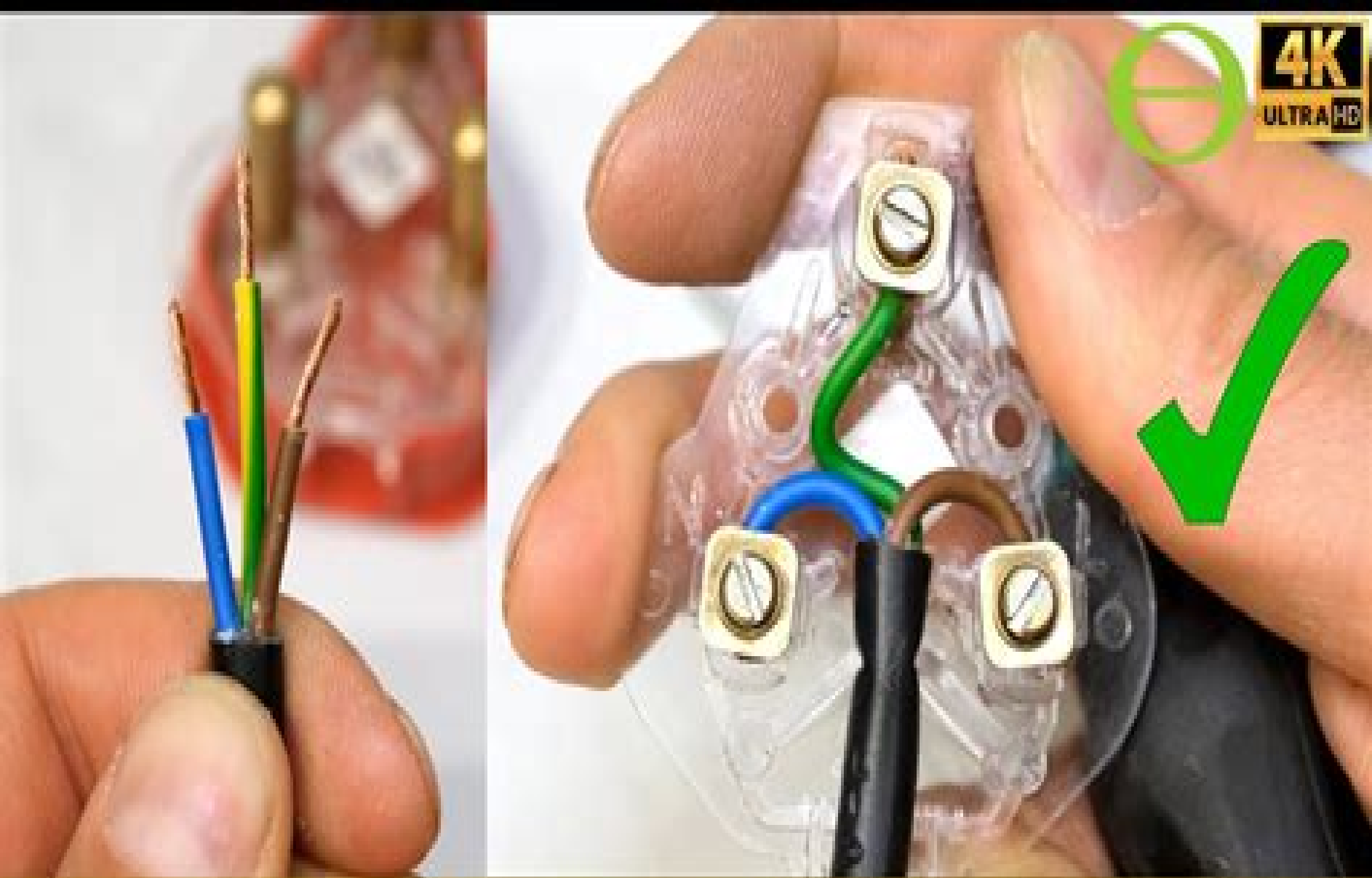
How to wire a South African plug
