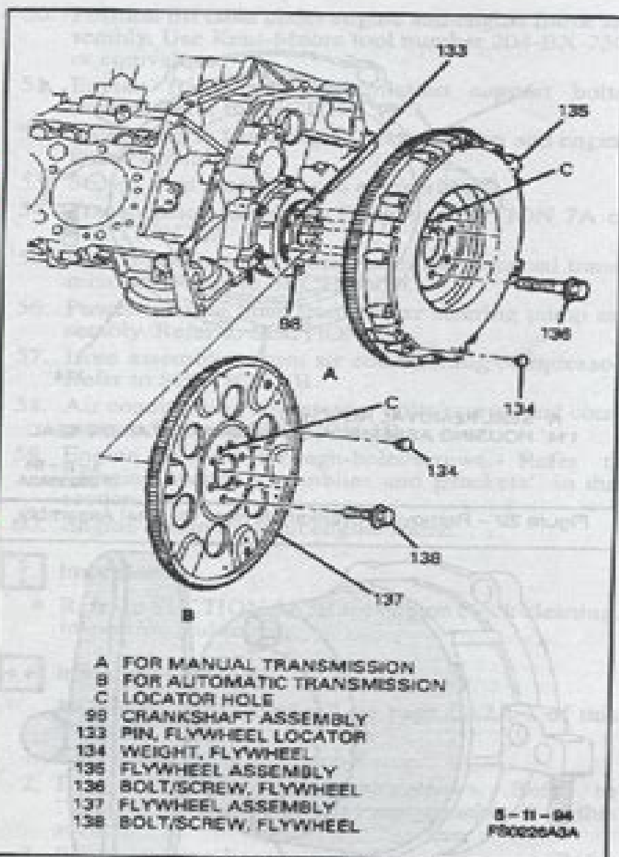
Figure 28 – Flywheel Assembly
