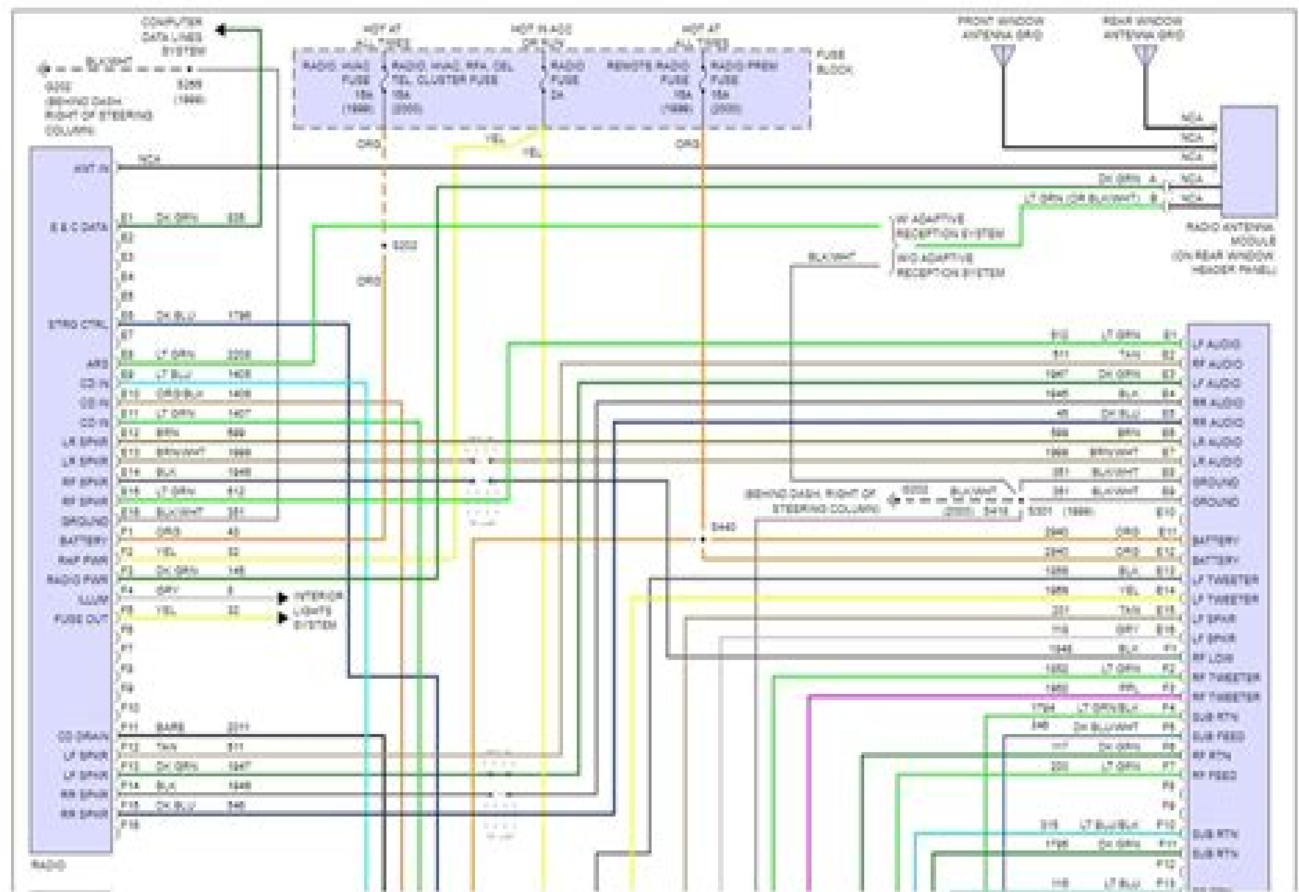
Fig 1: Radio Circuits, W/ Amplifier
